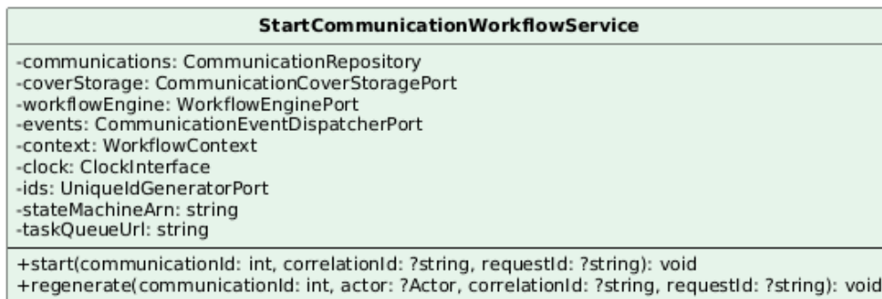
Figura 55: Classe — StartCommunicationWorkflowService
