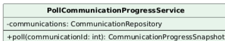
Figura 59: Classe — PollCommunicationProgressService
