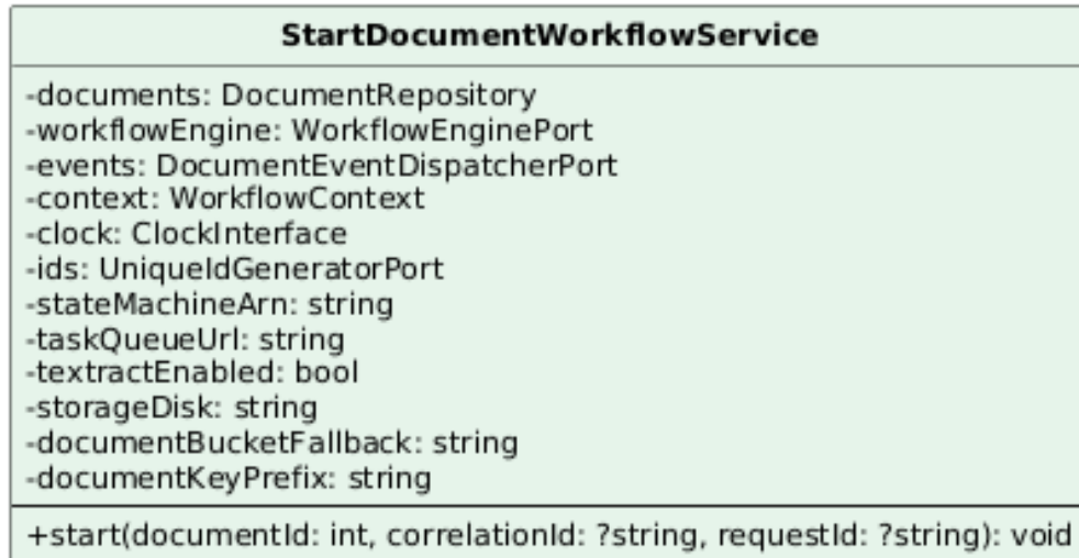
Figura 21: Classe — StartDocumentWorkflowService
